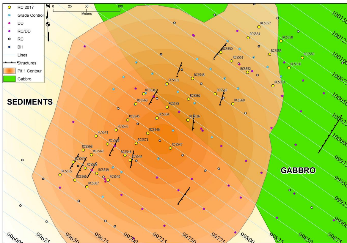
Figure 2: Makabingui Pit 1 drilling location plan
